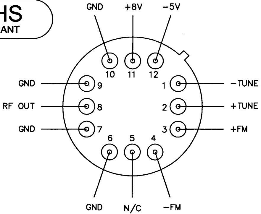
PINOUT
